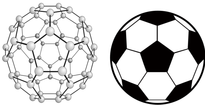
Figure 1: Structure of C_{60} molecule discovered by Kroto, Curl and Smalley compared to that of a football/soccer ball containing 12 pentagons and 20 hexagons: a truncated icosahedron structure
