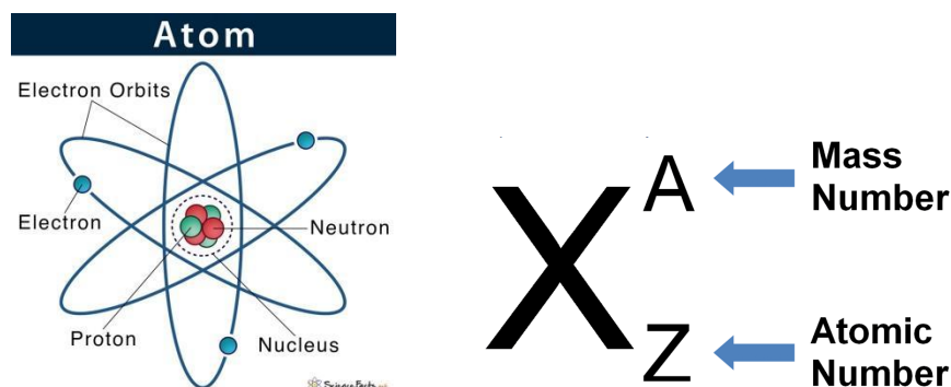
Figure 1: Structure of an atom Figure 2: Representation of mass number and atomic number
