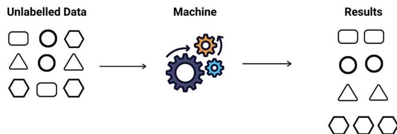
Figure 3: Unsupervised learning
