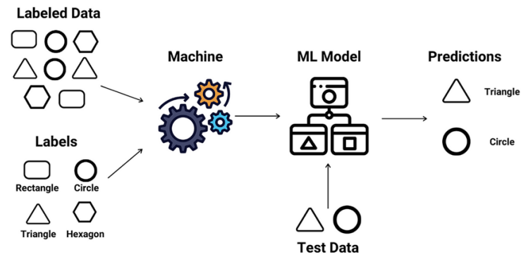
Figure 2: Supervised learning
