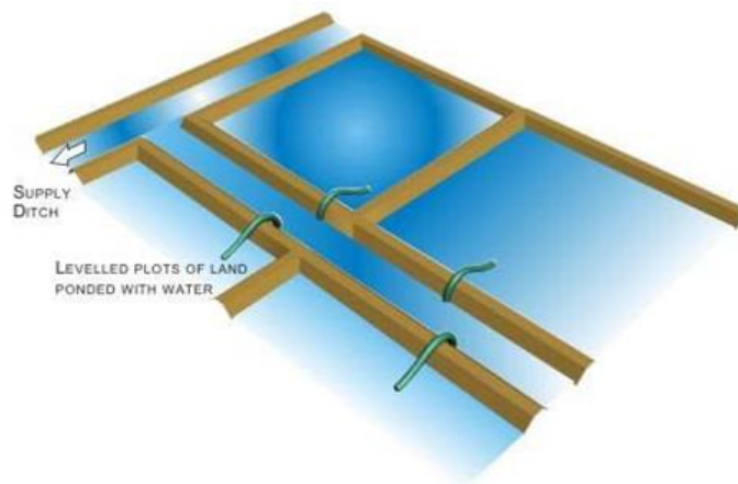
Figure 1: Layout of check basin irrigation system
