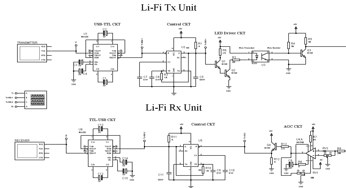
Figure 3: Combined Li-Fi Transmitter and Receiver
