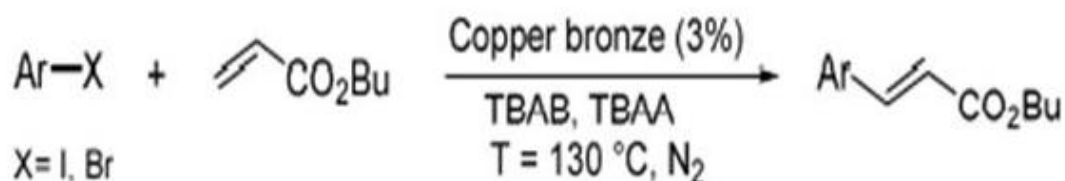
Figure 5. Copper nanocolloids in presence of TBAB, TBAA for the Heck reaction.
