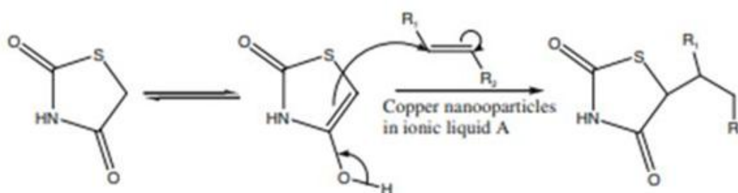
Figure 1. Michael addition reaction in presence of copper NPs in IL A
