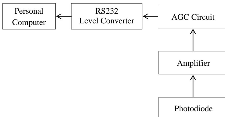
Figure 2: Components of Li-Fi Receiver System
