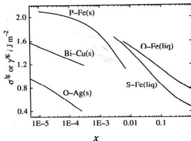
Figure 3: Surface tension in solid Fe, Cu, and Ag near their melting temperatures [5] and liquid Fe at 1550–1600 °C [2] as a function of concentration for certain surface-active organisms
