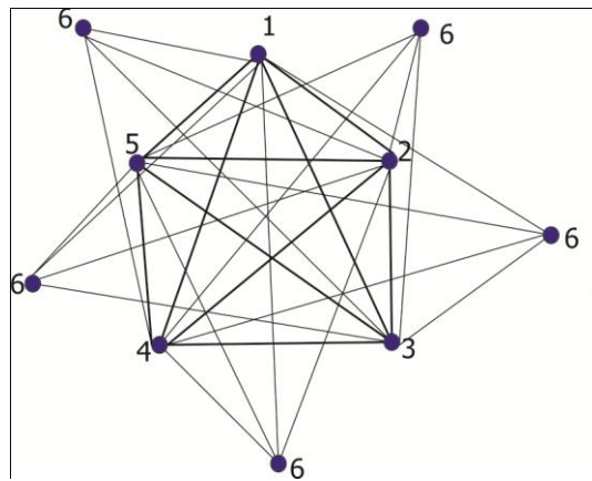
Figure 3: \psi[S(K_5)] = 6, n \geq 3 .
