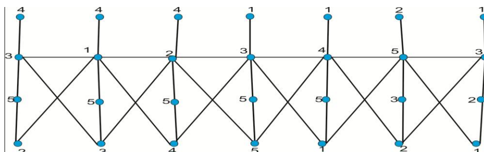
Figure 4: \phi[S(Cb_7)] = 5
