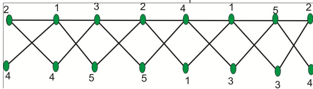
Figure 1: \varphi[S(P_8)] = 5
